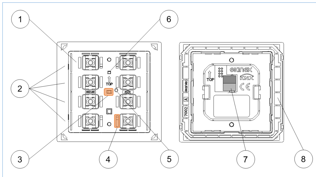
Figure 2 – Switching, display and connection elements
